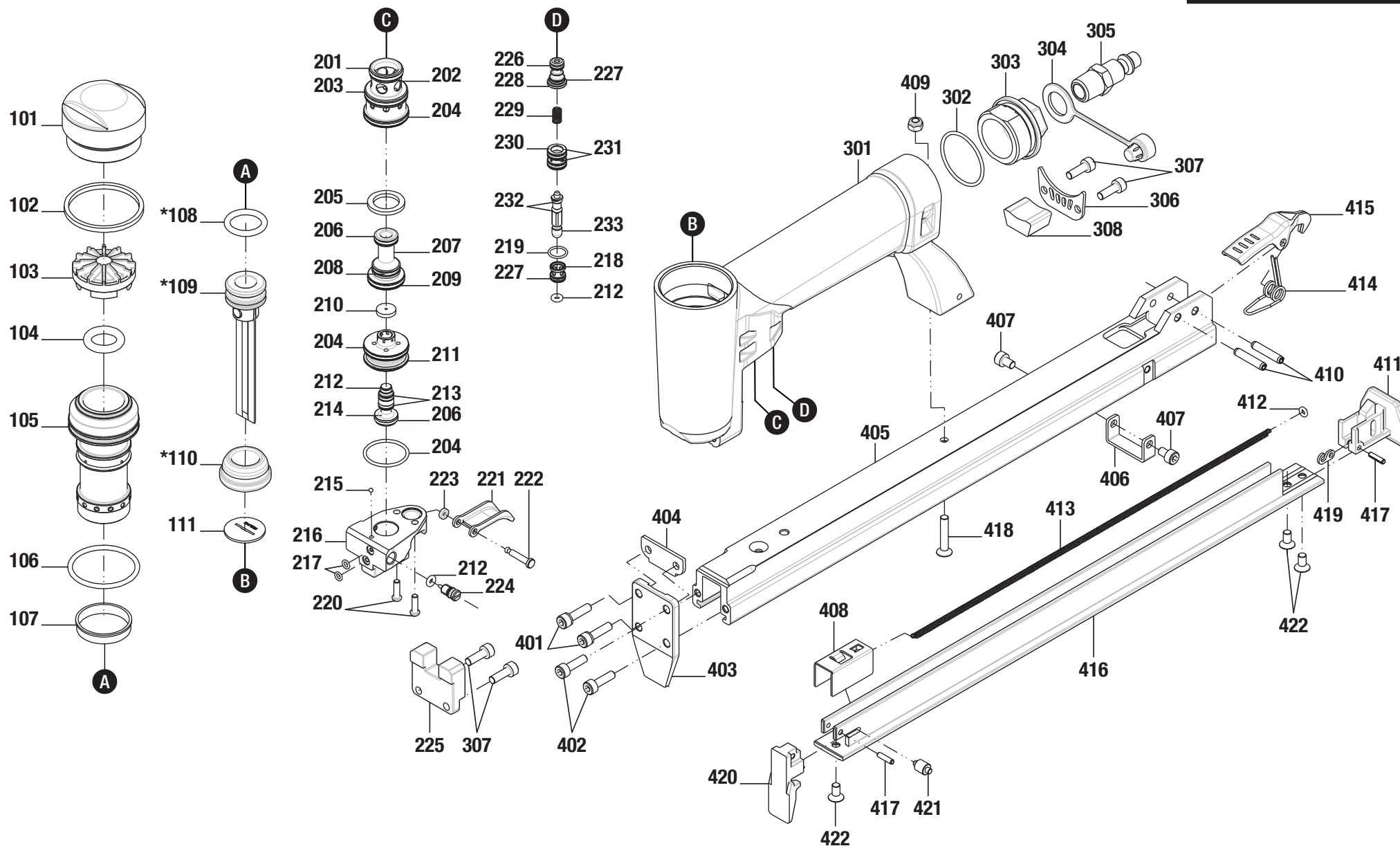
simG80 LM | Explosionado - Exploded view
