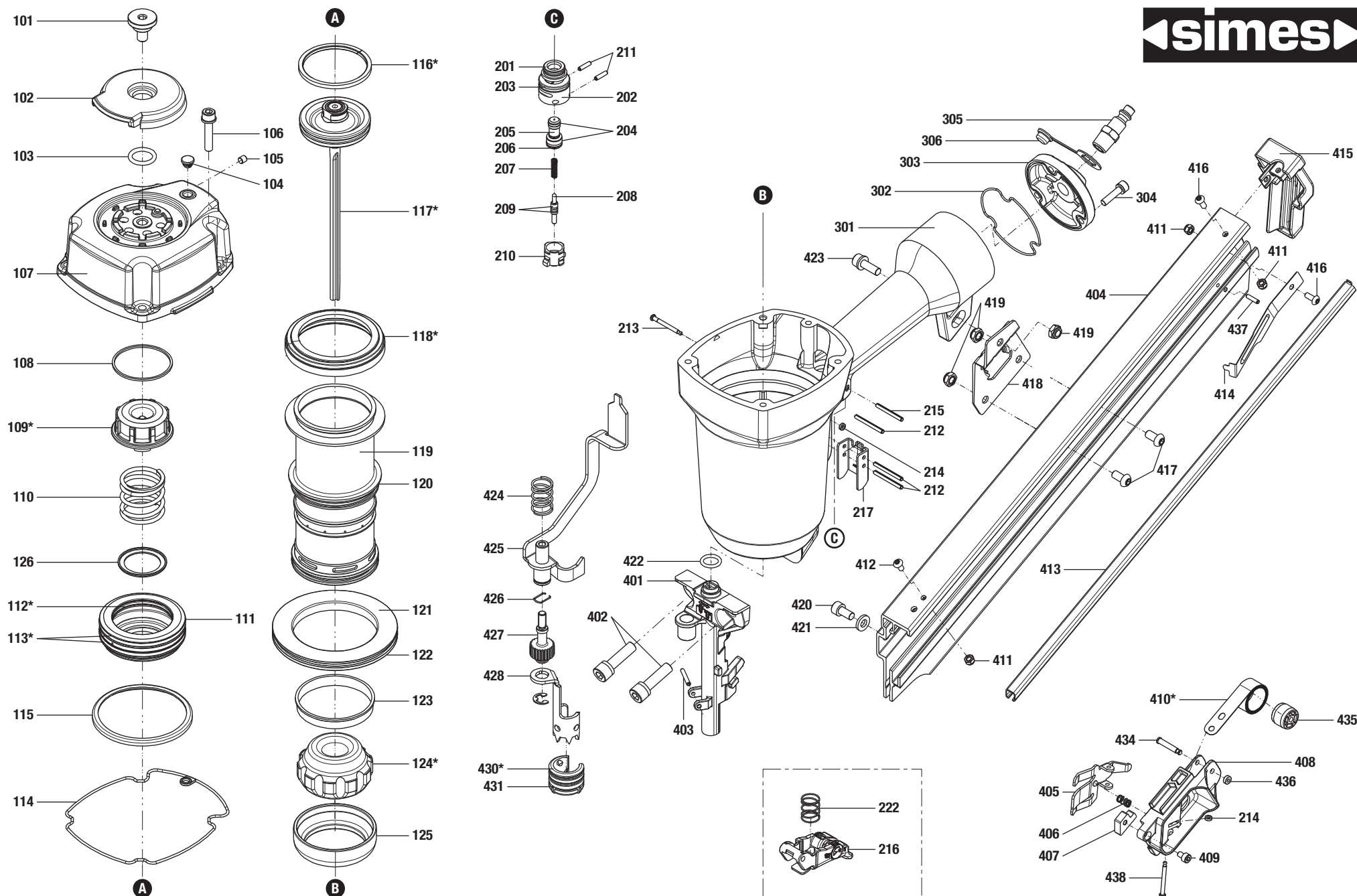
simHF90 | Explosionado - Exploded view
