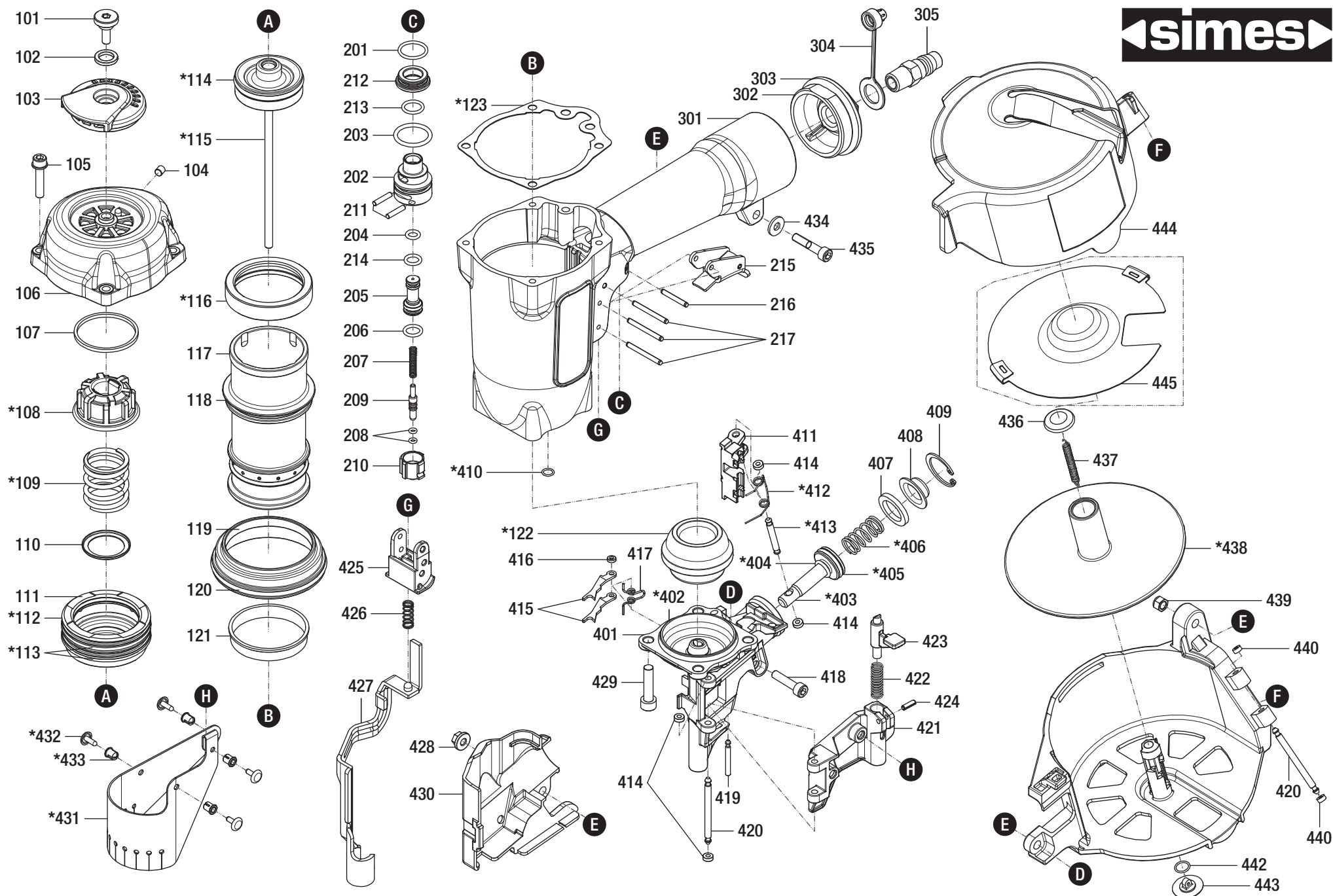
simC50 | Explosionado - Exploded view
